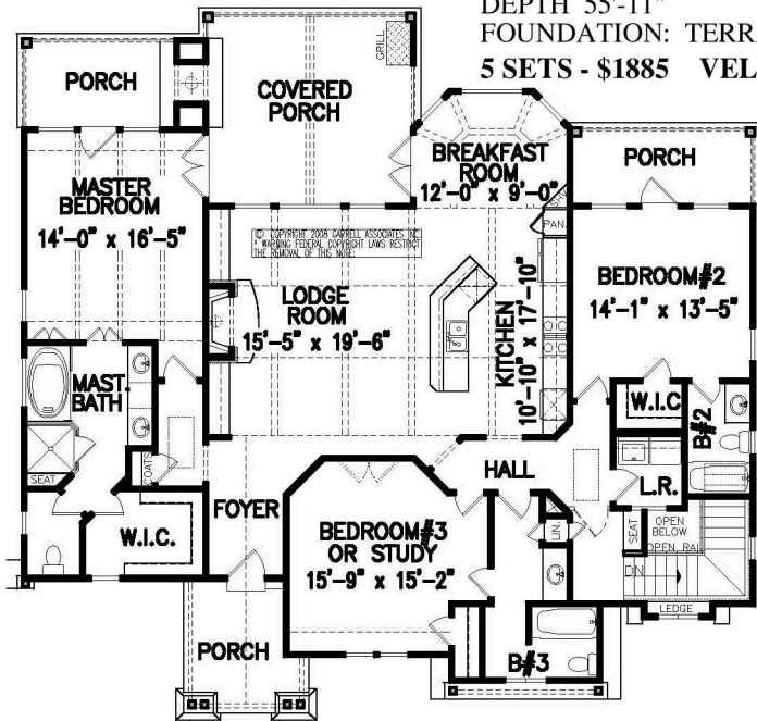
FIRST FLOOR PLAN 2,091 SQ. FT.
