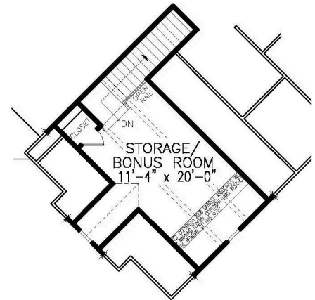
OPTIONAL SECOND FLOOR PLAN BONUS ROOM: ADDITIONAL 290 SQ. FT.
