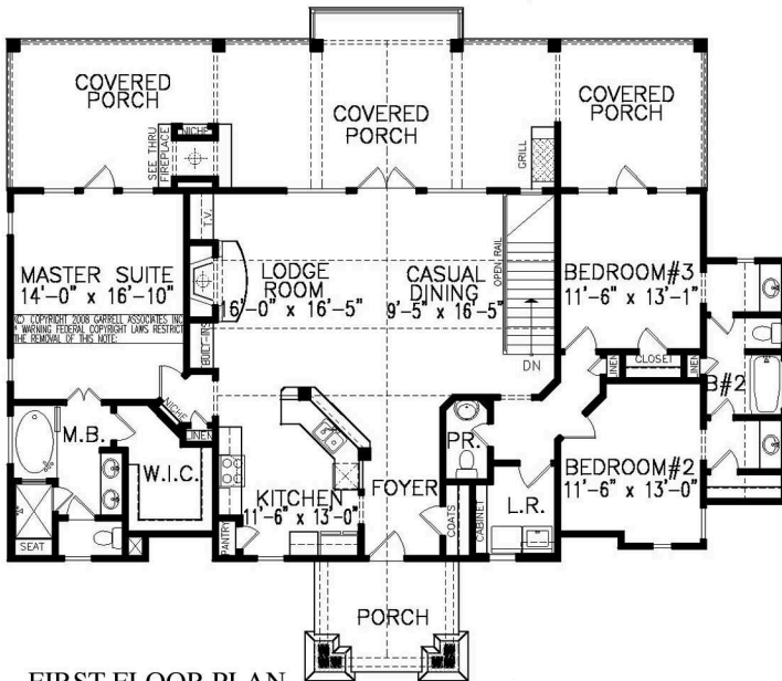
FIRST FLOOR PLAN 1,792 SQ. FT.
