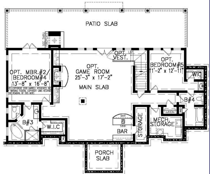
OPTIONAL BASEMENT PLAN ADDITIONAL 1,546 SQ. FT. MECH./STORAGE 135 SQ. FT.
