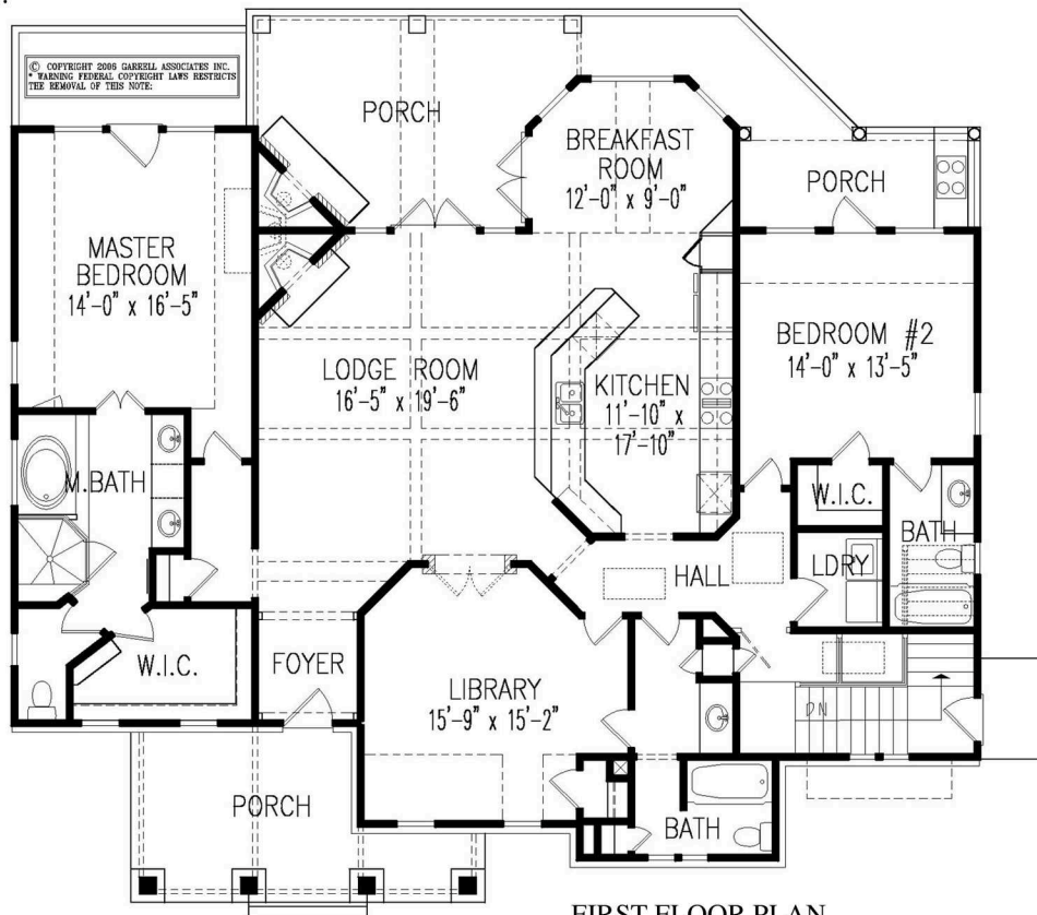
FIRST FLOOR PLAN 1,997 SQ. FT.
